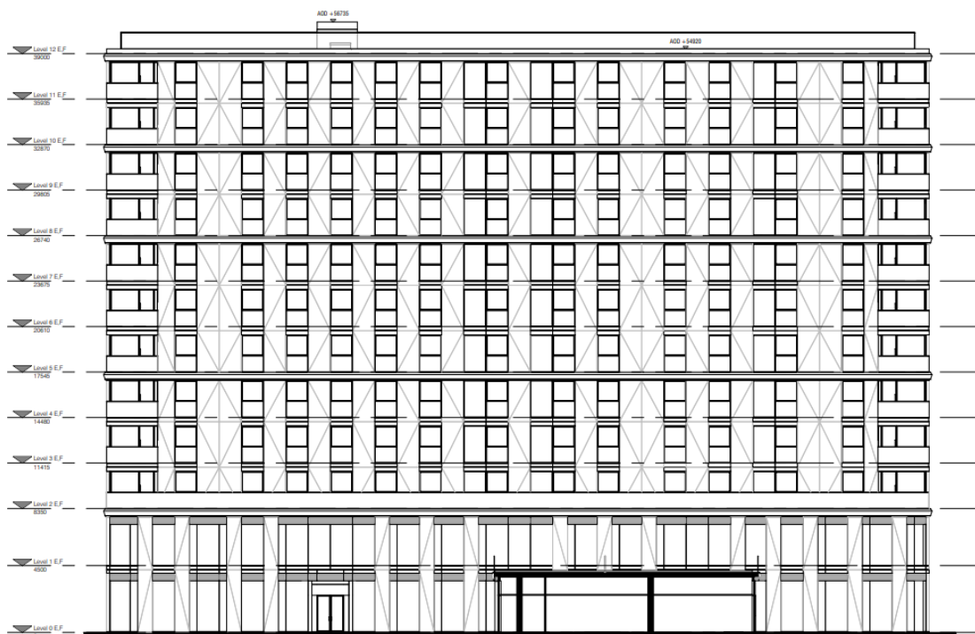
Block F Northern Elevation
