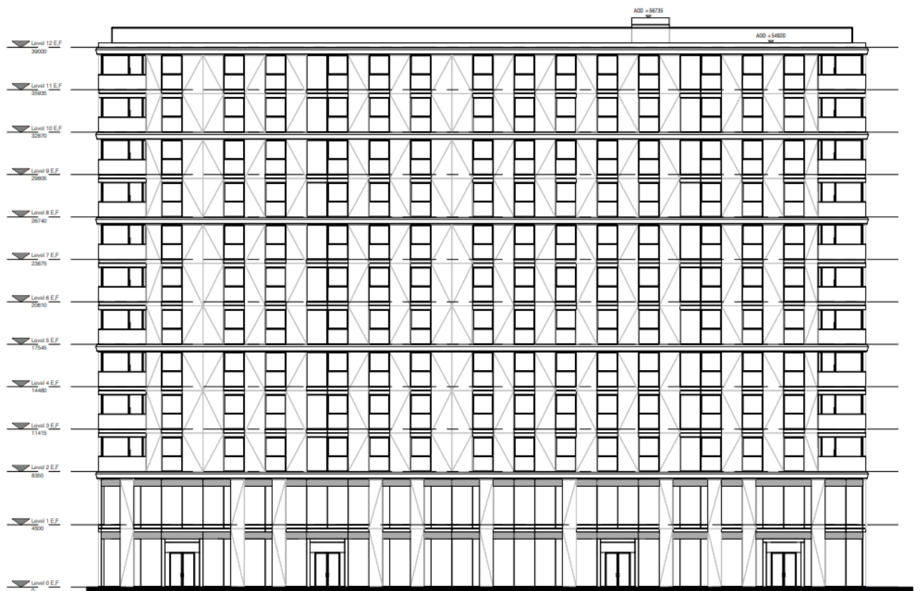
Block F London Road Elevation (South)
