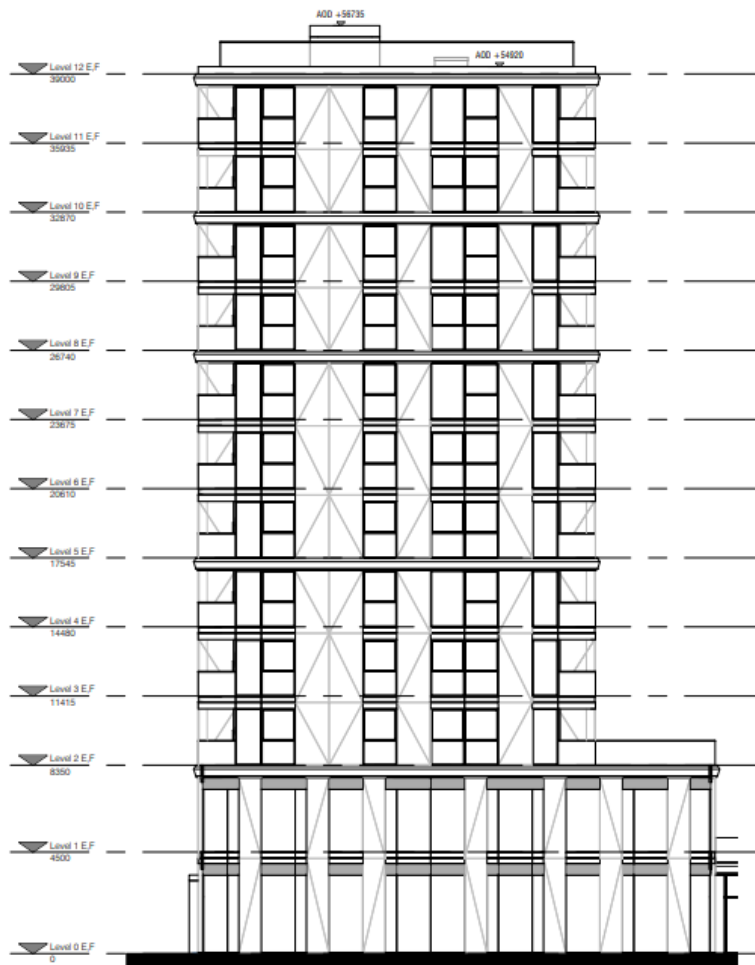
Block F Eastern Elevation
