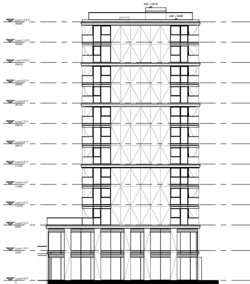
Block F Western Elevation
